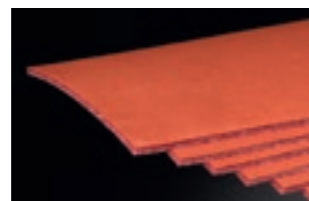
Filler mat PGUDLQHILLERMAT, 6.37 m 2 26 mats / box. Used for the space between the heating mats and the wall.
