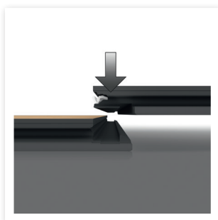
Drop down (not available for rigid click)
