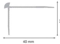
Stair nose, outer PGVSTPGLUE, 2000 x 40 x 26 mm
