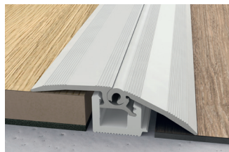
Combi moulding, aluminium PGPRSILV, 1860 x 10 x 47 mm
